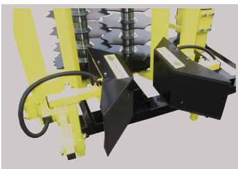
Magnetic sensors - open and close cutting heads when sensing steel posts
